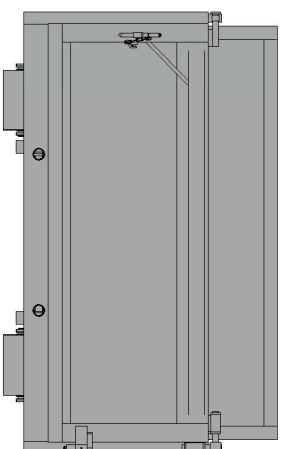
CLC12/6000G Combined top and side opening door with manual locking
