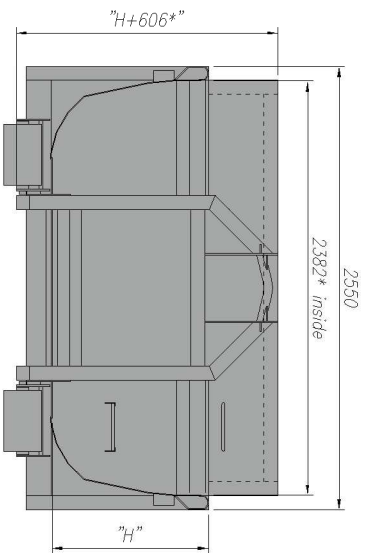
CLC12/6000D Combined top and side opening door with pneumatic/hydraulic flap locking
