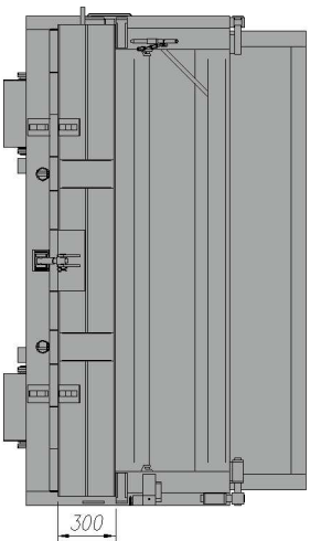
CLC12/6000D Combined top and side opening door with pneumatic/hydraulic flap locking
