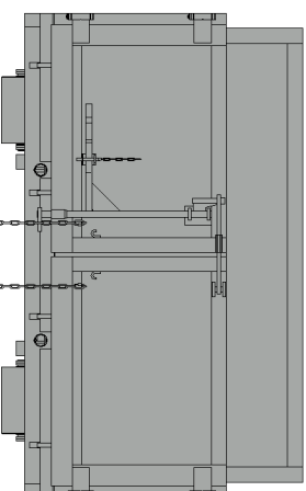
CLC12/6000HDD2 Top hinged frame with hydraulic opening double door and manual locking
