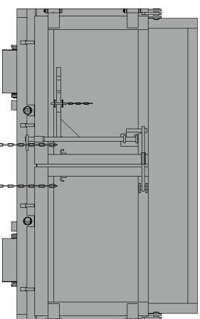
CLC12/6000GD Double door with top hinge opening and manual locking
