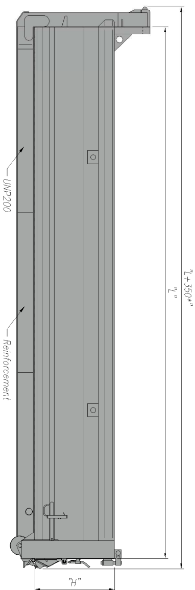
CLC12/6000G Combined top and side opening door with manual locking
