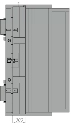
CLC12/6000HDD Hydraulic opening top hinged door with flap locking
